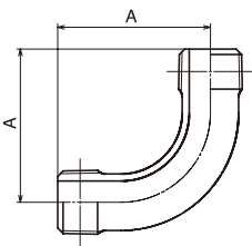
Bends 90° Male * Fig.035
