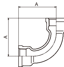
Bends 90° Bended Female * Fig.036B
